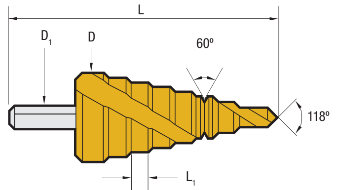
Spiral Flute TiN Step Drills
