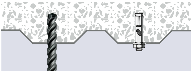
Deltagon SDS-Plus Masonry Bits easily drill through Bondek® steel deck plate. Superior hole roundness results in increased anchor performance.
